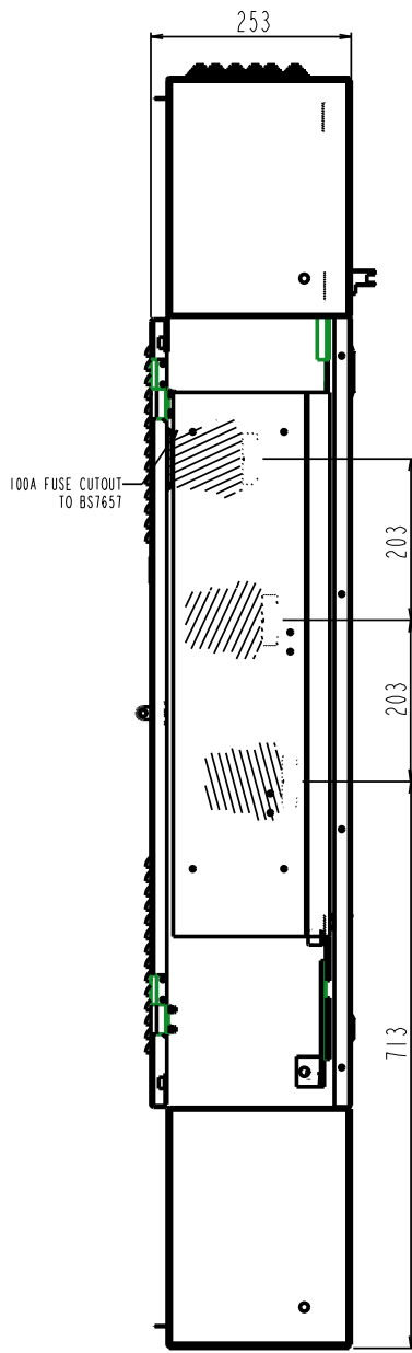
SECTION B-B SHOWING 100A FUSE CUTOUT
