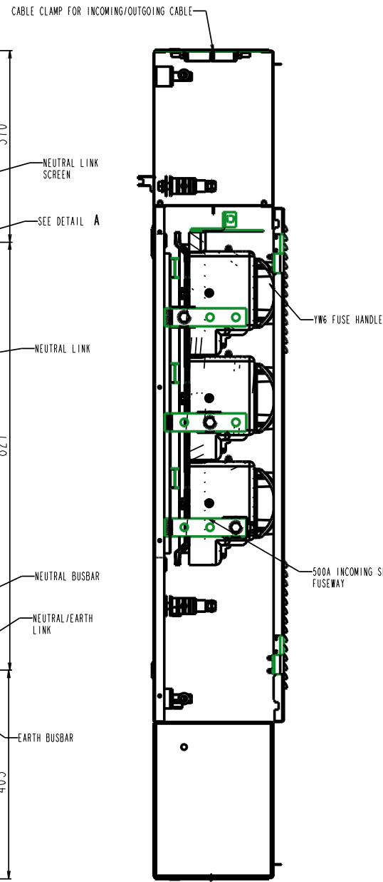
SECTION C-C SHOWING 500A INCOMING SHIELDED FUSEWAY
