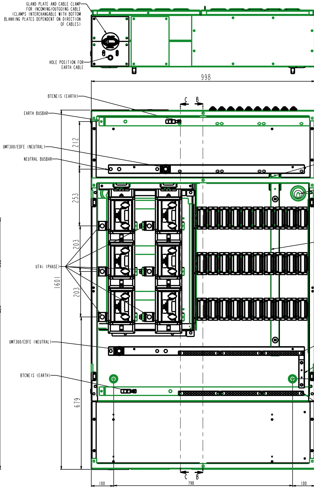
FRONT VIEW WITH DOOR AND INCOMING/OUTGOING CABLE SCREENS REMOVED
