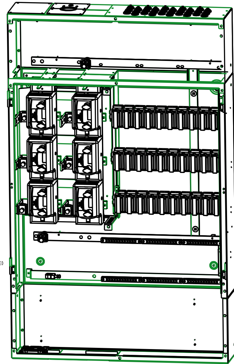
ISOMETRIC FRONT VIEW WITH DOOR REMOVED
